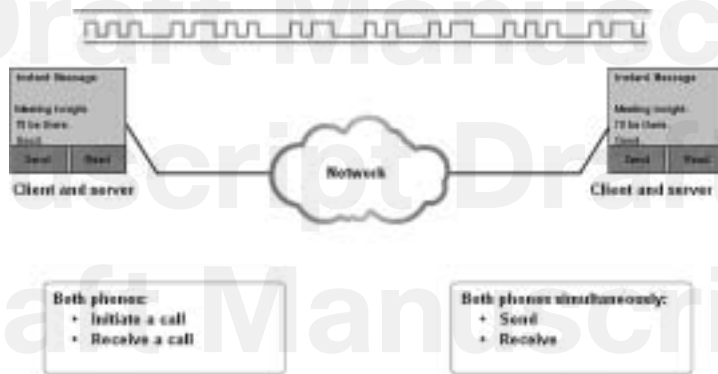
Figure 3-10 Peer-to-Peer Applications
