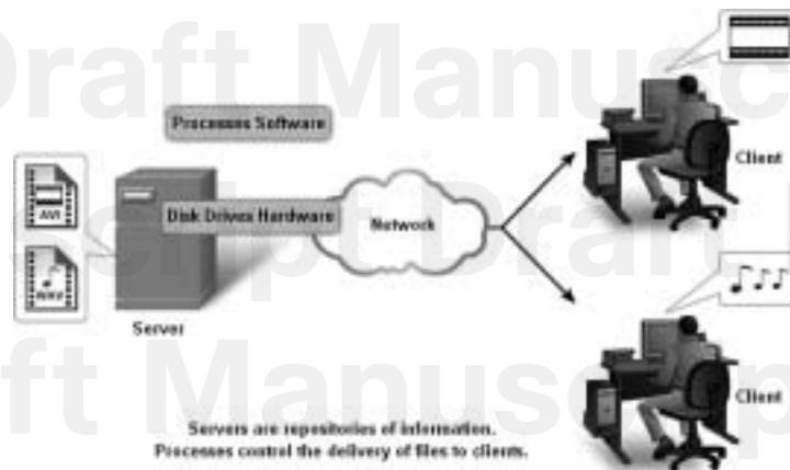
Figure 3-7 Servers
