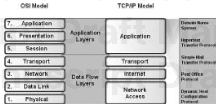
Figure 3-3 OSI and TCP/IP Model
