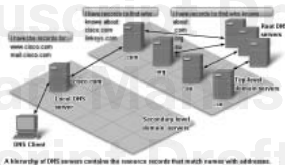
Figure 3-12 DNS Server Hierarchy
