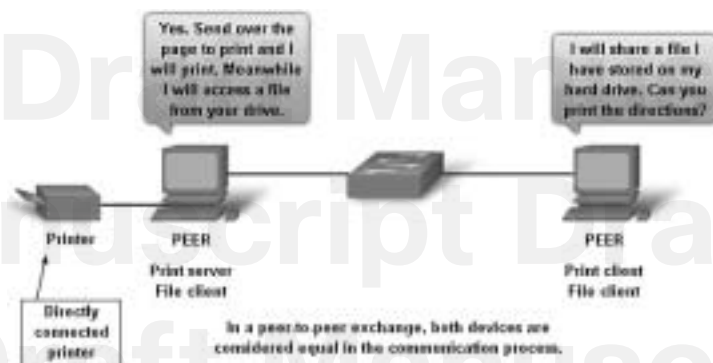
Figure 3-9 Peer-to-Peer Networking
