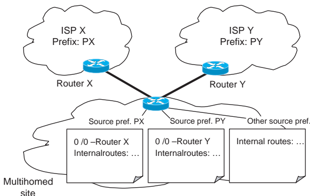
Fig. 3. SAD routing.
