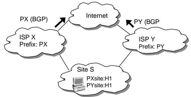
Fig. 2. Provider aggregation of end-site prefixes.
