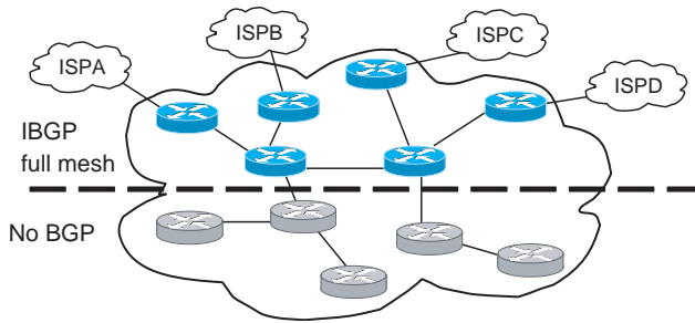
Fig. 5. IBGP full mesh.
