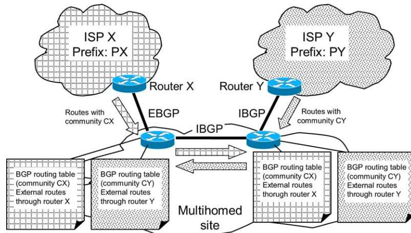
Fig. 6. SAD routing deployment using BGP communities.
